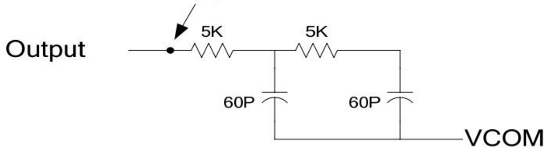
Output load condition
