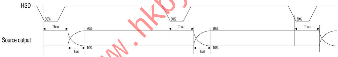
Source output timing diagram
